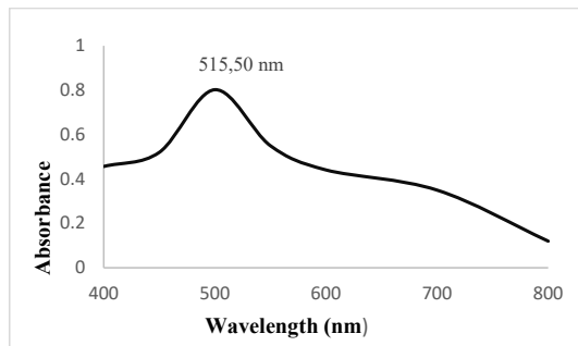
Figure 2. DPPH Wavelength
