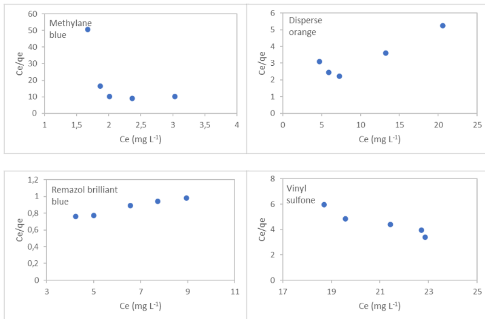
Figure 2. Langmuir sorption isotherms of dyes onto coral reef.
